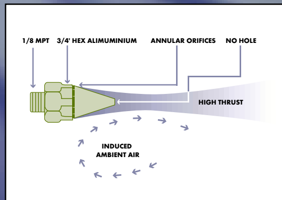
HOW THE AIRMISER WORKS
