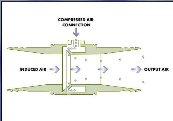
HOW THE RING JET AIR CONVEYORS WORKS
